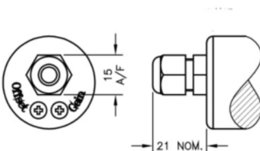
Cable gland, IP67, Option L:
