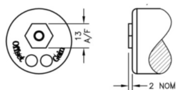
Short Cable Gland, IP67, Option M,
