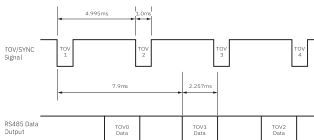
Figure 7.4 Timing Diagram
