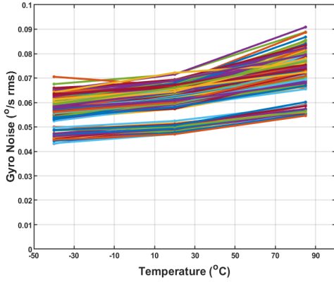
Figure 5.7 Gyro Noise (°/s rms) vs Test Chamber Temperature
