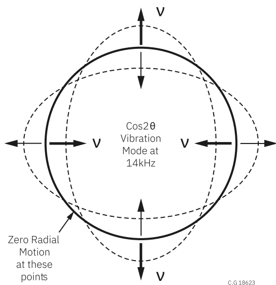
Figure 12.3 Primary Vibration Mode
