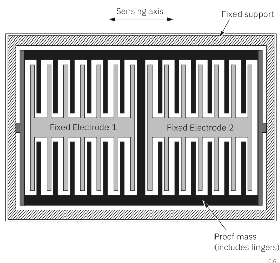
Figure 12.5(a) Schematic of Accelerometer Structure
