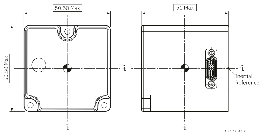
Figure 11.2 Position of the Inertial Reference Point
