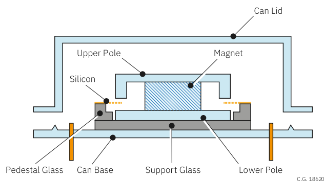
Figure 12.2 MEMS VSG3Q MAX Sensor
