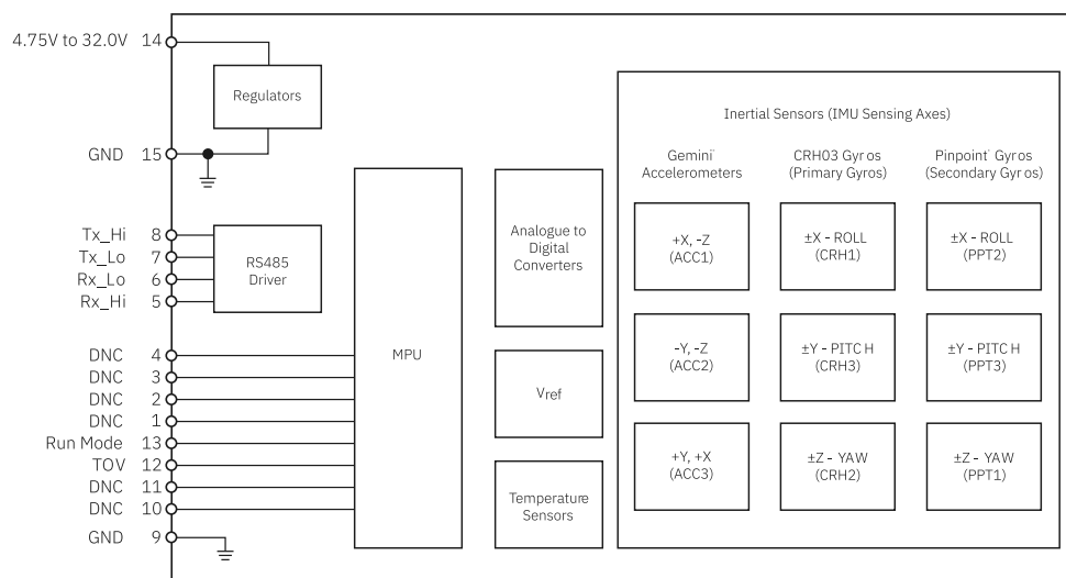
Figure 1.1 DMU41 Functional Block Diagram
