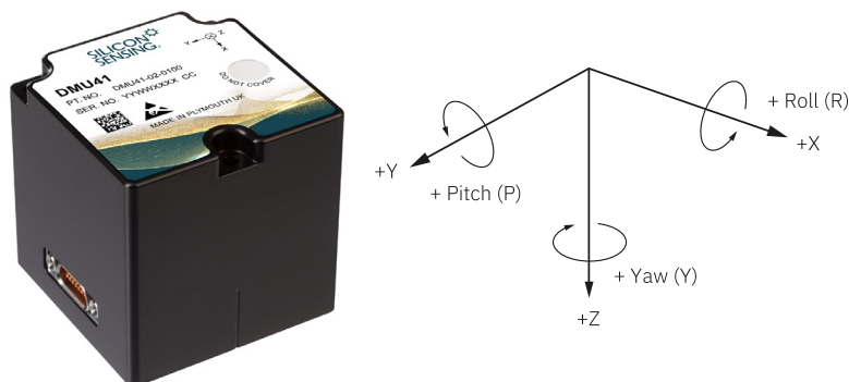
Figure 11.1 Axis Definitions
