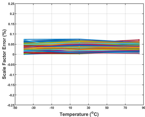
Figure 5.11 Accelerometer Scale Factor Error ( \pm 1g range) over Temperature (Plymouth g = 9.81058m/s/s )
