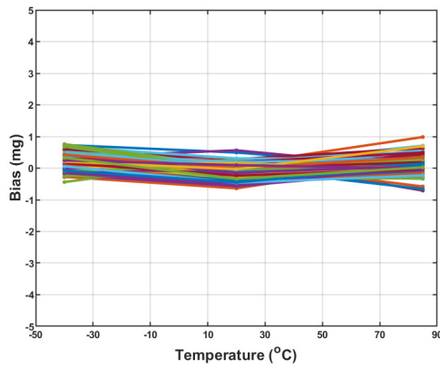
Figure 5.9 Accelerometer Bias Error (mg) over Temperature
