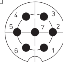
Male connector front view
