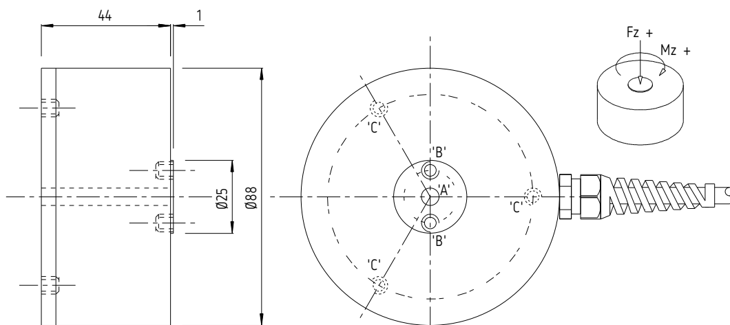
'A' Ø6 THRO. 'B' M6x1 ON A 18 PCD - 2 OFF. 'C' M6x1 EQUI SPACED ON A 70 PCD - 3 OFF
