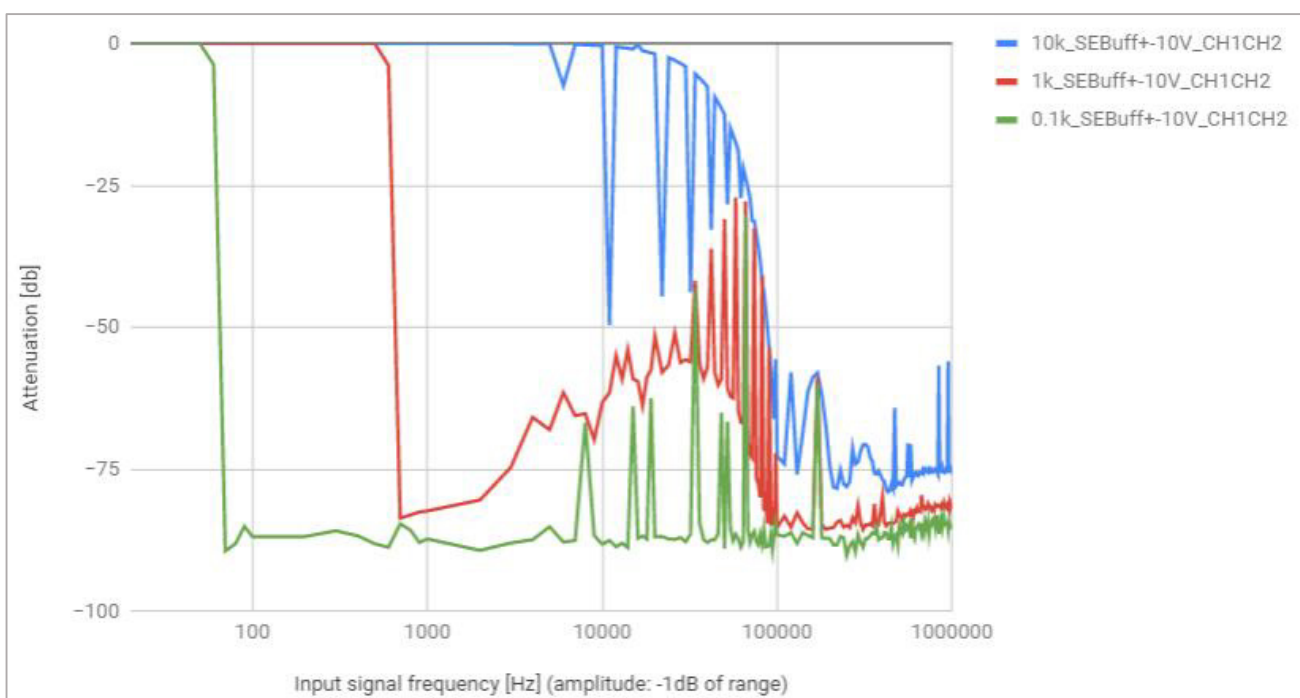
Analog input frequency response – multi channel mode (mux), buffered single-ended input, different sample rates
